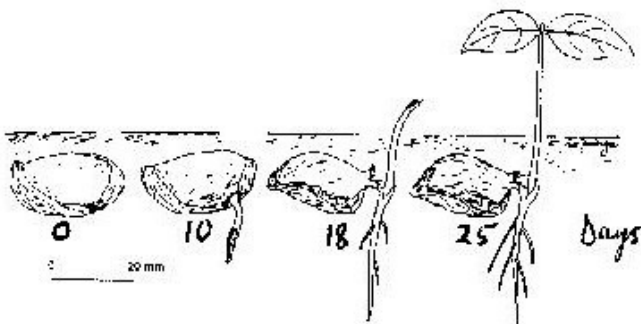
Stages in the Germination of Khaya senegalensis seed
